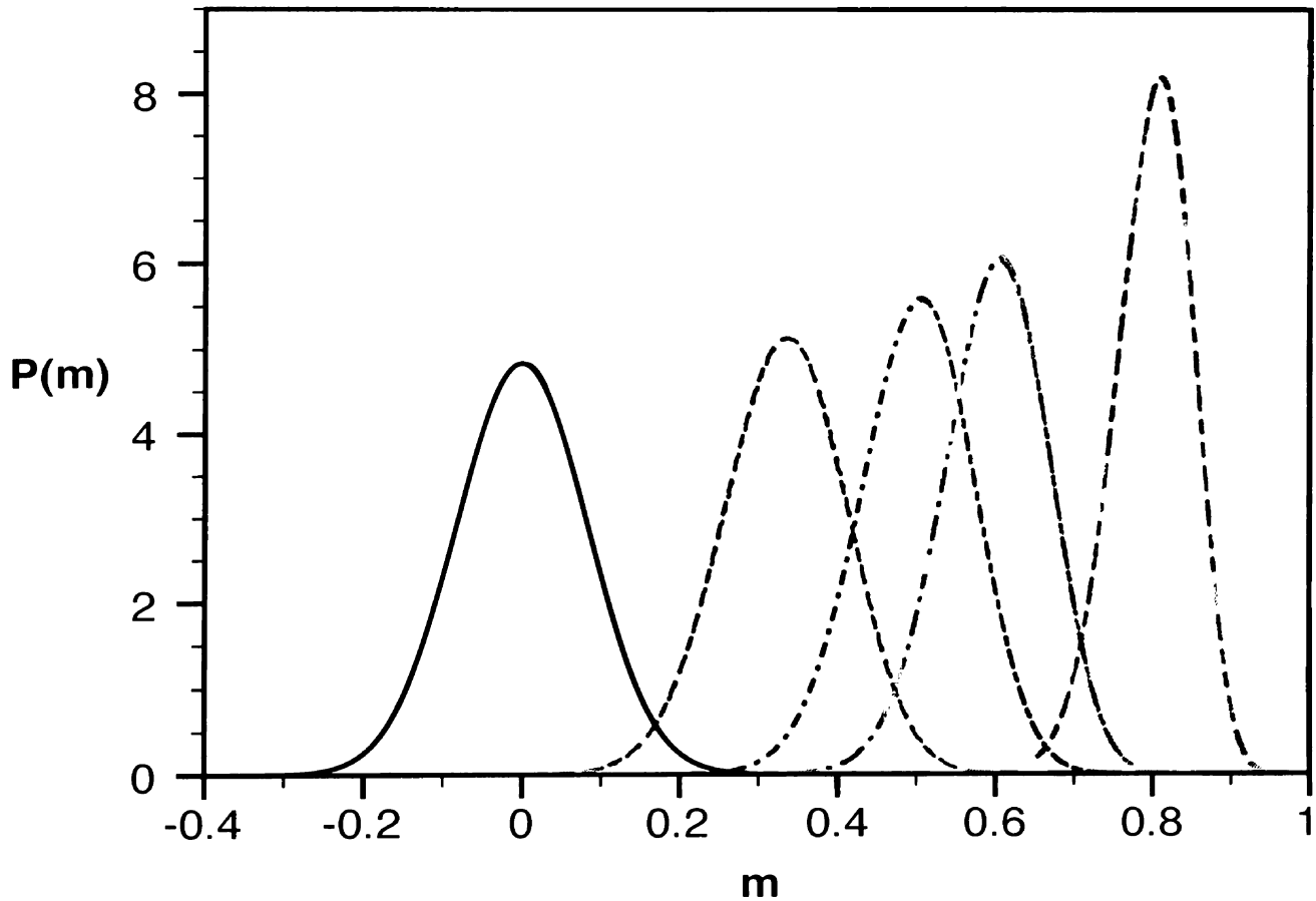
Figure 9.2: Steady-state magnetization distributions on a complete graph of 1000 sites with unequal numbers of zealots. Shown left to right are the cases of (Z_+, Z_-) = (90, 90), (120, 60), (135, 45), (144, 36), (162, 18) . The results of voter model simulations and the solution to the master equations are coincident. The mean magnetization of the system equals the magnetization of the zealots: m = \frac{z_+ - z_-}{z_+ + z_-} .
