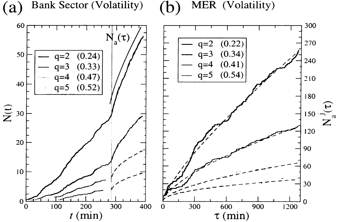
Figure 3.5: The Omori law relaxation can extend for several days. We compare the Omori exponents \Omega_a(q) (indicated in legends) calculated for (a) the time series N_a(\tau) of the Bank sector and (b) the time series N_a^j(\tau) of Merrill Lynch for the three days (1275 minutes) after the announcement on Tuesday 08/21/01 at 2:15 pm ( \tau = 0 minutes corresponding to T = 285 minutes). For the remaining 3 days of the trading week, the Omori law relaxation corresponding to an individual stock (MER) is quantitatively similar to the the Omori law relaxation of the Bank sector over the final 105 minutes of the initial trading day. We do not use the Bank sector N_a(\tau) over the same 1275-minute time period for comparison because “opening effects” occurring during the first 60 minutes of each trading day makes power-law regression of conjoined N_a(\tau) problematic.
