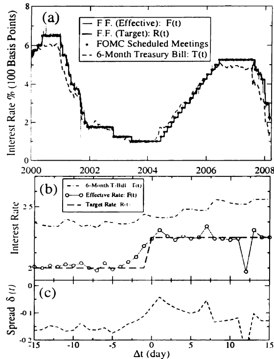
Figure 3.1: An illustration of the close relation between the Treasury Bill and the Federal Funds rate. (a) Time series of the Federal Reserve Target rate, R(t) , and the Federal Reserve Effective rate, F(t) , for Federal Funds (F.F.) dating from Jan. 2000 to Apr. 2008. The 6-Month Treasury Bill, T(t) , tends to anticipate the effective rate, with speculation about future changes causing deviations in the relative values. United States Treasury Bills carry little risk, and are considered to be one of the most secure investments. (b) A typical illustration of the Federal Funds Effective rate and the Treasury Bill, where both gravitate around the Federal Funds Target rate. The change in the relative spread \delta(t) , defined in Eq. (3.1), between the Treasury bill and the Federal Funds Effective rate, indicates changes in market speculation. (c) The relative spread, \delta(t) , 15 days before and 15 days after the scheduled FOMC meeting on Dec. 14, 2004, which corresponds to \Delta t = 0 . Note that the average value of the relative spread increases after the announcement, indicating a shift in market consensus and speculation.
