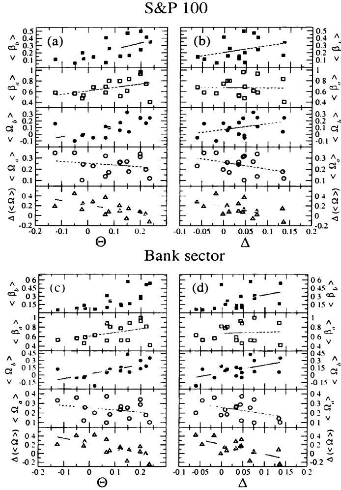
Figure 3.9: The relation between the size of the financial shock, quantified by the S&P 100 volatility Omori law parameters \langle \beta_b \rangle , \langle \beta_a \rangle , \langle \Omega_b \rangle , \langle \Omega_a \rangle , and \Delta(\langle \Omega \rangle) = \langle \Omega_a \rangle - \langle \Omega_b \rangle , and the size of the FOMC news, quantified through the metrics \Theta representing market anticipation and \Delta representing market surprise. All trends are consistent with the hypothesis that a strong anticipation of an interest rate change, and the element of surprise inherent in the FOMC decision, result in a market perturbation that is significant in scale, and broad across the market. Linear regressions of S&P100 data (a,b) and bank sector data (c,d) are provided for visual aide. Linear regressions that pass the ANOVA F-test (rejecting null hypothesis that regression slope m = 0 ) at the \alpha = 0.05 significance level are solid; regressions that fail to pass the F-test at the \alpha = 0.05 significance level are dashed.
