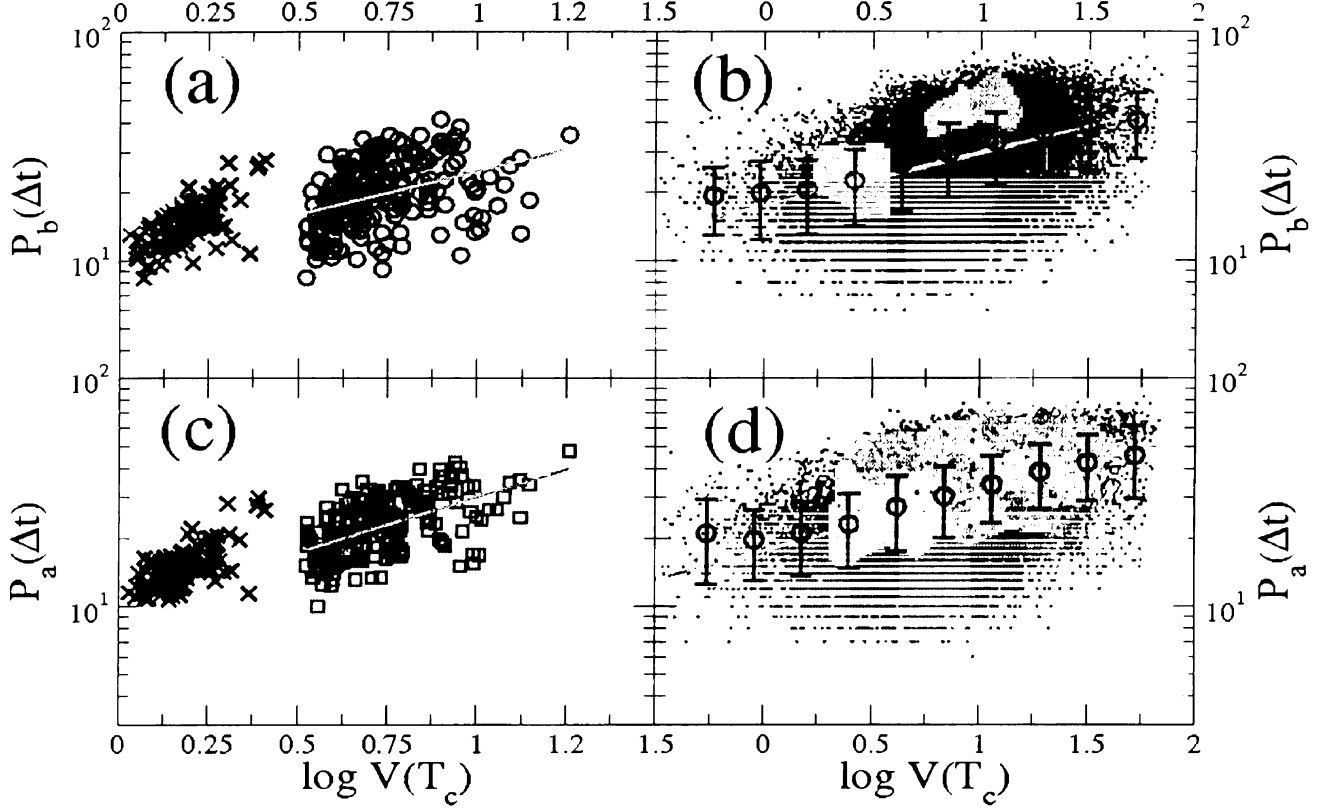
Figure 4.10: The increasing relation between the productivity P_{a,b}(\Delta t) of each market shock and the size of the main shock M \equiv \log V(T_c) with \Delta t \equiv 90 min. As is found in earthquakes, we find a power-law relationship between M and V(T_c) described by a productivity exponent \Pi_b before and exponent \Pi_a after the market shock. Data points in panels (a) and (c) denoted by the symbol \times correspond to values of P_{a,b}(\Delta t) calculated for randomly selected T_c on those 118 days analyzed without a single value of x(t) > x_c . The result that P(\Delta t) increases with increasing V(T_c) holds even for random times. For the average market response N_{b,a}(\Delta t) , we find (a) \Pi_b = 0.38 \pm 0.07 and (c) \Pi_a = 0.48 \pm 0.04 . For the productivity of individual stocks corresponding to N'_{b,a}(\Delta t) we find (b) \Pi_b = 0.23 \pm 0.01 and (d) \Pi_a = 0.25 \pm 0.01 . For comparison, the power-law exponent value pertaining to earthquake aftershocks is \Pi_a \approx 0.7 - 0.9 [60].
