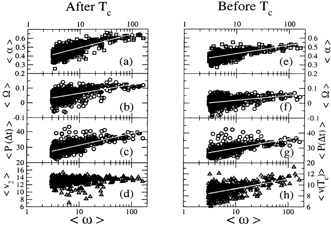
Figure 4.13: Relations between individual stock trading activity and dynamic response parameters (a-d) after T_c and (e-h) before T_c , averaged over all the days with a market shock. We measure the trading activity \langle \omega \rangle for each stock, defined as the average number of transactions per minute over the 2-year period 2001-2002. We find that stocks with large trading activity react both more strongly (larger \alpha and larger P(\Delta t) ) and quickly (larger \Omega ) to market shocks. However, panel (d) shows that there is little relation between \langle \omega \rangle and the average size of the largest aftershock \langle v_2 \rangle .
