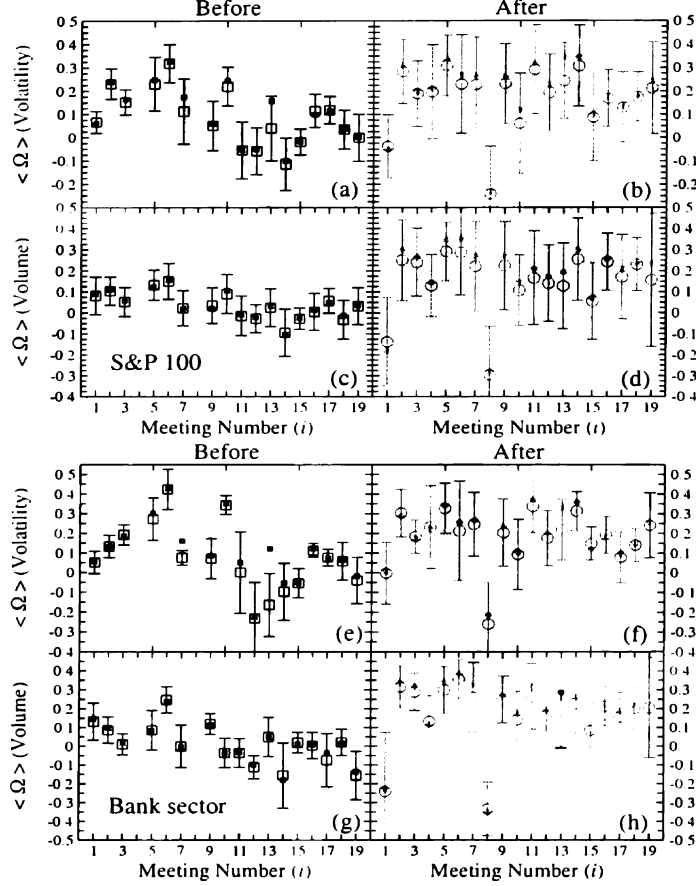
Figure 3.7: Comparison of Omori law exponents for both volatility dynamics and volume dynamics on the day of 19 FOMC meetings during the two-year period Jan. 2001- Dec. 2002. Panels (a-d) correspond to the S&P 100 and panels(e-h) correspond to the bank sector. The similarity in exponents for 1-minute volatility and 1-minute cumulative volume suggest a universal underlying mechanism. Solid symbols ( \blacksquare and \bullet ) refer to \Omega computed from N(t) . Open symbols ( \square and \circ ) refer to \langle \Omega \rangle computed from S individual Omori exponents \Omega^j , with S_{bank} = 18 . Note the relatively low value of \Omega_a and \langle \Omega_a \rangle for unscheduled FOMC announcements i = 1 and 8, which indicates that volatility rate following the announcement increased throughout the day.
