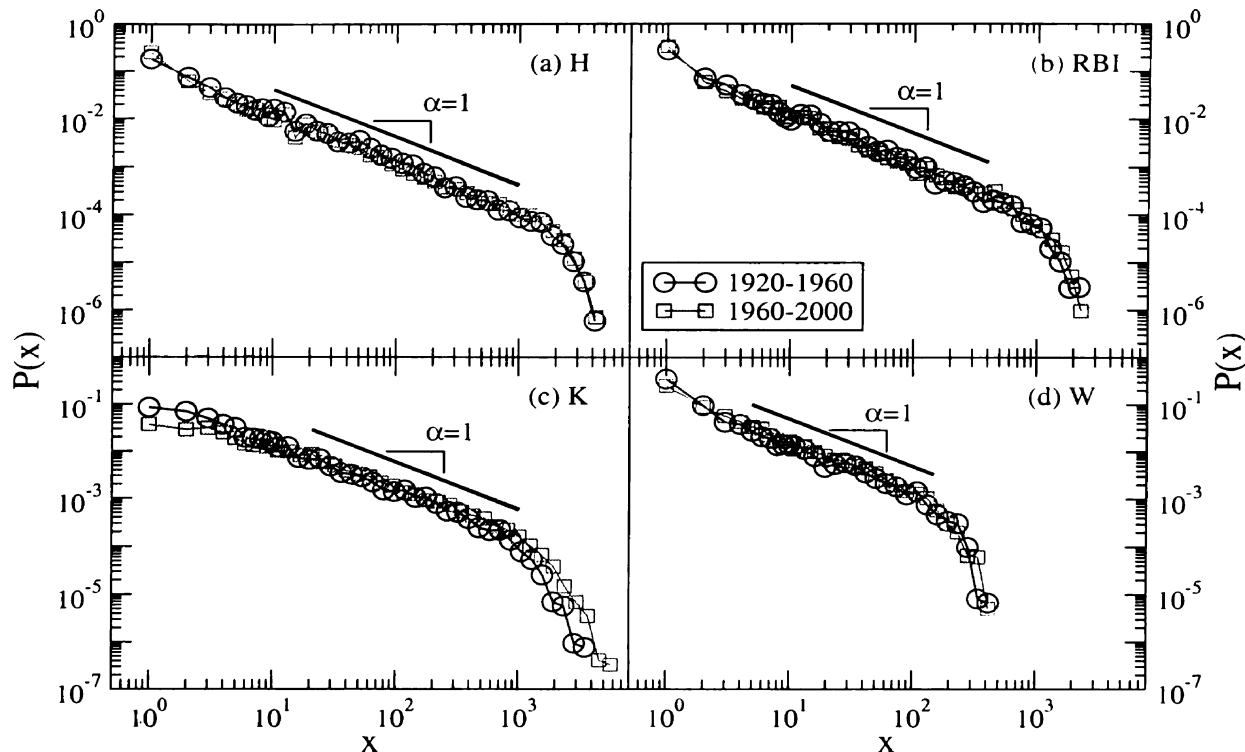
Figure 6.2: Probability density function of career statistics in four categories. (a) Hits, (b) Runs Batted In, (c) K (strikeouts). (d) Wins. Plotted for each statistical metric are the distribution of career totals for players whose career ended in the periods 1920-1960 and 1960-2000. The pairs of distributions are all qualitatively similar, with the exponential cutoffs occurring at the same critical value, indicating that the competition level in baseball has been relatively constant with respect to these career metrics.
