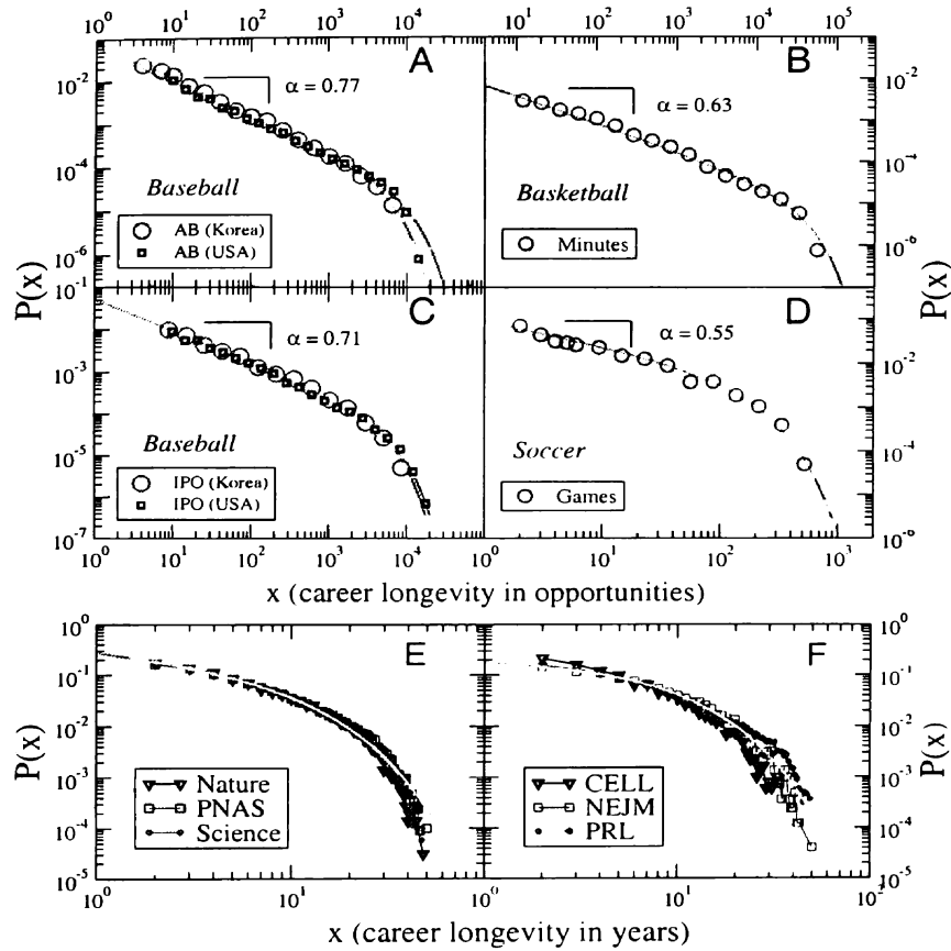
Figure 7.3: Extremely right-skewed pdfs P(x) of career longevity in several high-impact scientific journals and several major sports leagues. Solid curves represent least-squares best-fit functions corresponding to the functional form in Eq. [7.5]. (A) Baseball fielder longevity measured in at-bats (pitchers excluded): we find \alpha \approx 0.77 , x_c \approx 2500 (Korea) and x_c \approx 5000 (USA). (B) Basketball longevity measured in minutes played: we find \alpha \approx 0.63 , x_c \approx 21000 minutes. (C) Baseball pitcher longevity measured in innings-pitched measured in outs (IPO): we find \alpha \approx 0.71 , x_c \approx 2800 (Korea), and x_c \approx 3400 (USA). (D) Soccer longevity measured in games played: we find \alpha \approx 0.55 , x_c \approx 140 games. (E and F) High-impact journals exhibit similar longevity distributions for the “journal career length” which we define as the duration between an author’s first and last paper in a particular journal. Deviations occur for long careers due to data set limitations (for comparison, least-square fits are plotted in panel (E) with parameters \alpha \approx 0.40 , x_c = 9 years and in panel (F) with parameters \alpha \approx 0.10 , x_c = 11 years).
