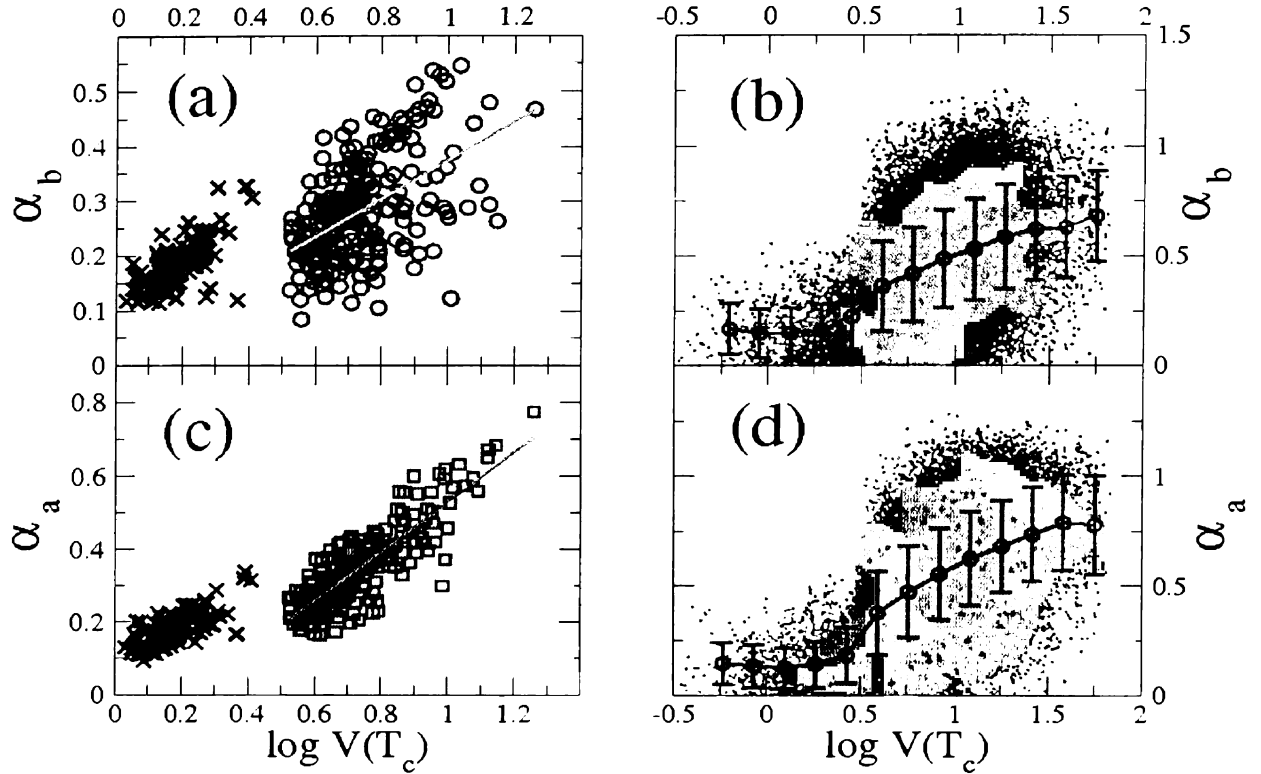
Figure 4.9: The relation between the magnitude M \equiv \log V(T_c) and the Omori amplitudes \alpha_{a,b} . In panels (a) and (c) we compare the values calculated from the average market response N(\tau) and in panels (b) and (d) we compare values calculated from individual stock response N_{a,b}^j(\tau) . (a) The increasing relation between \alpha_b and M is statistically stronger than the relation between \Omega_b and M in Fig. 4.8(a), with significance p \approx 0 , correlation coefficient r = 0.52 and regression slope m = 0.35 \pm 0.04 . (c) The relation between \alpha_a and M is strong, with significance p \approx 0 , r = 0.84 , and regression slope m = 0.68 \pm 0.03 . Data points in panels (a) and (c) denoted by the symbol \times correspond to values of \alpha_{a,b} calculated for randomly selected T_c on those 118 days analyzed without a single value of x(t) > x_c . The result that \alpha increases with increasing V(T_c) holds even for random times. In panels (b) and (d) there is much dispersion in the \alpha values of individual stocks for given V(T_c) . However the average trends demonstrate a significant crossover at M_x \approx 0.5 from \alpha_{a,b} \approx 0.2 for M < 0.5 to \alpha_{a,b} > 0.2 for M > 0.5 . This crossover occurs at a similar location as the crossover observed in Figs. 4.8(b) and (d) for \Omega_{b,a} . The average amplitude value \bar{\alpha} increases sharply for M > M_x , consistent with first order phase transition behavior.
