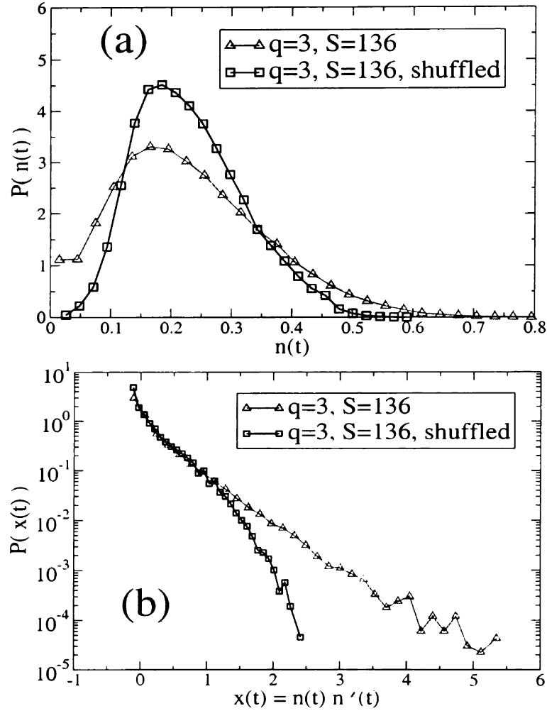
Figure 4.5: Using the volatility threshold q = 3 and S = 136 stocks, we determine the market co-movement threshold x_c from the pdf of x(t) \equiv n(t)n'(t) . (a) The pdf for the 190,000 minutes analyzed of the volatility rate n(t) corresponding to the fraction of the market with volatility v_i(t) > q . (b) The pdf of x(t) , where in the quantity x(t) we have removed the average daily trend of n(t) , so that x(t) is relatively large when market co-movement is large and significant. For comparison, we also plot the pdf of x_{sh}(t) computed from randomly shuffled volatility time series v_i(t) . We find a divergence between the pdf of x(t) and of x_{sh}(t) for x > 1.0 , which we define as the co-movement threshold x_c \equiv 1 in our analysis.
