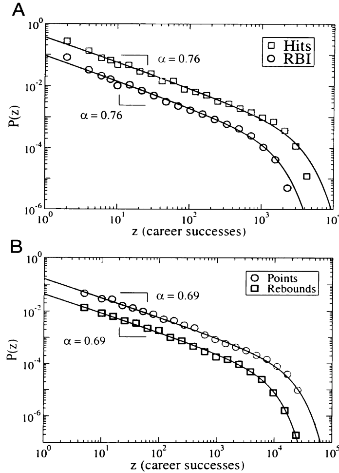
Figure 7.4: Probability density function P(z) of common metrics for career success, z . Solid curves represent best-fit functions corresponding to Eq. [7.5]. (A) Career batting statistics in American baseball: x_c^{Hits} \approx 1200 , x_c^{RBI} \approx 600 . (RBI = Runs Batted In). (B) Career statistics in American basketball: x_c^{Points} \approx 8000 , x_c^{Rebounds} \approx 3500 . For clarity, the top set of data in each plot has been multiplied by a constant factor of four in order to separate overlapping data.
