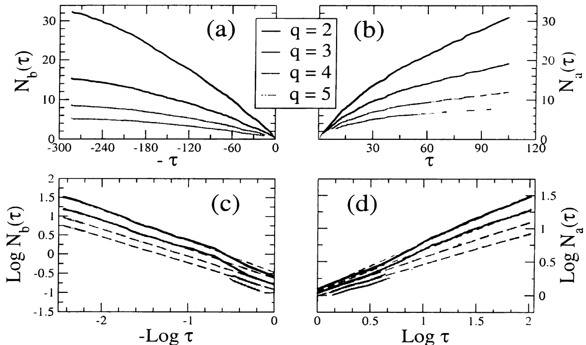
Figure 3.6: An illustration of the method used to calculate (a) N_{b,i}(\tau) = N_i(T_i) - N_i(|t - T_i|) and (b) N_{a,i}(\tau) = N_i(t - T_i) - N_i(T_i) for each intraday time series N_i(t) . The displaced time \tau = |t - T_i| is defined symmetrically around the time of the announcement T_i . We plot the same data as in Fig. 3.4 (a), corresponding to the announcement on 05/15/01 which occurred at T = 285 minutes. Panels (c) and (d) show that N_{b,i}(\tau) and N_{a,i}(\tau) are approximately linear on logarithmic scale.
