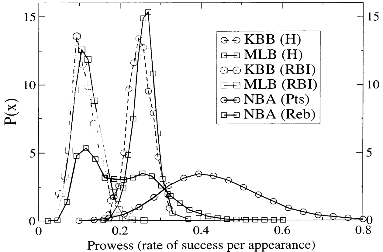
Figure 7.5: Probability density functions of seasonal prowess for several career metrics. Each pdf is normally distributed, except for the bimodal curve for rebound prowess. NBA (Reb.). The bimodal distribution for Rebound prowess reflects the specialization in player positions in the sport of basketball. Furthermore, note the remarkable similarity in the distributions between American (MLB) and Korean (KBB) baseball players.
