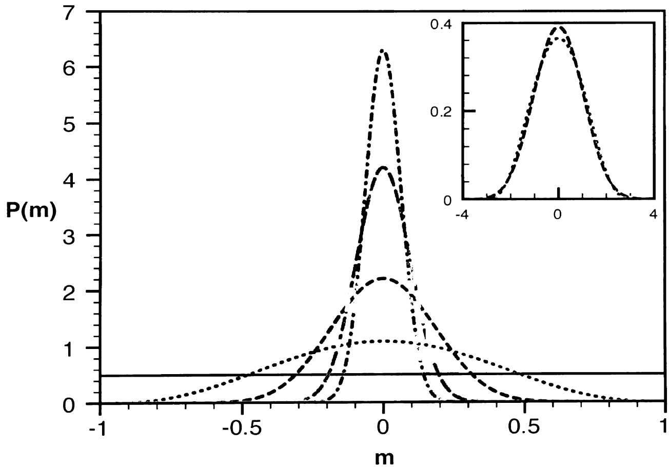
Figure 9.1: Steady-state magnetization distributions for 1000 voters on the complete graph for Z = 2, 8, 32, 128, and 512 zealots (progressively steepening curves). The inset shows the scaled form of these distributions for Z \geq 8 ; the case Z = 8 slightly deviates from the rest of the distributions that become visually coincident.
