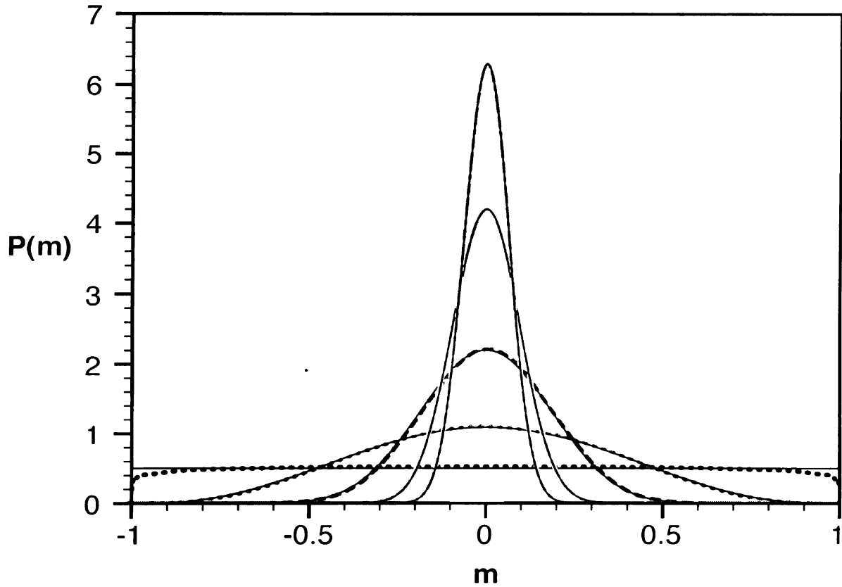
Figure 9.6: Comparison of simulations for the magnetization distribution in two dimensions (dashed) with the mean-field results (solid curves). The simulations are for 1000 voters with 2, 8, 32, 128 and 512 total zealots, with equal numbers of each type.
