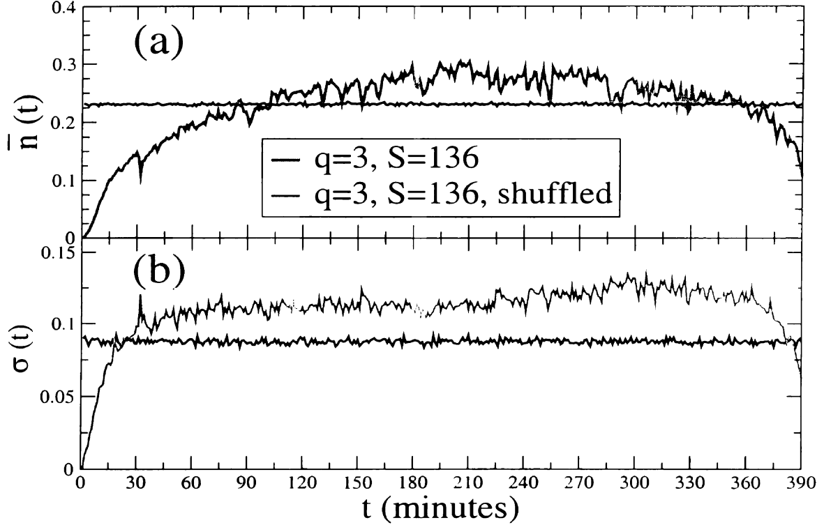
Figure 4.3: The fraction n(t) of the market above the volatility threshold q is non-stationary through the trading day. We plot in (a) the average daily trading pattern \bar{n}(t) for S = 136 stocks and in (b) the corresponding standard deviation. To demonstrate the trends we remove in the normalized quantity n'(t) . In practice, we use the smoothed average of these curves in order to diminish statistical fluctuations on the minute-to-minute scale. For comparison, we compute \bar{n}_{sh}(t) \approx 0.23 and \sigma_{sh} \approx 0.09 for shuffled v_i(t) . The values of \bar{n}(t) provide an estimate for the background market co-movement that can be attributed to random fluctuations.
