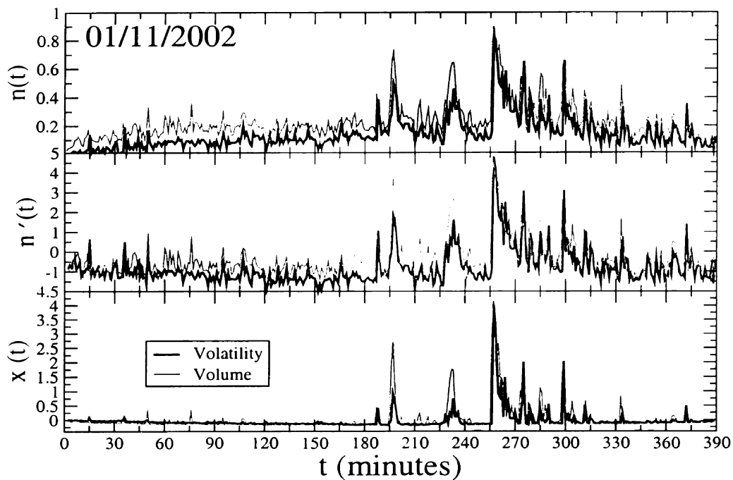
Figure 4.4: Example of market co-movement n(t) in both price volatility and total volume, and the qualitative relationship between the quantities n(t) , n'(t) \equiv (n(t) - \bar{n}(t))/\sigma(t) , and x(t) \equiv n(t)n'(t) . The market shock on 01/11/2002 occurred at T_c = 256 in response to a public comment by the Fed chairman A. Greenspan concerning economic recovery [53].
