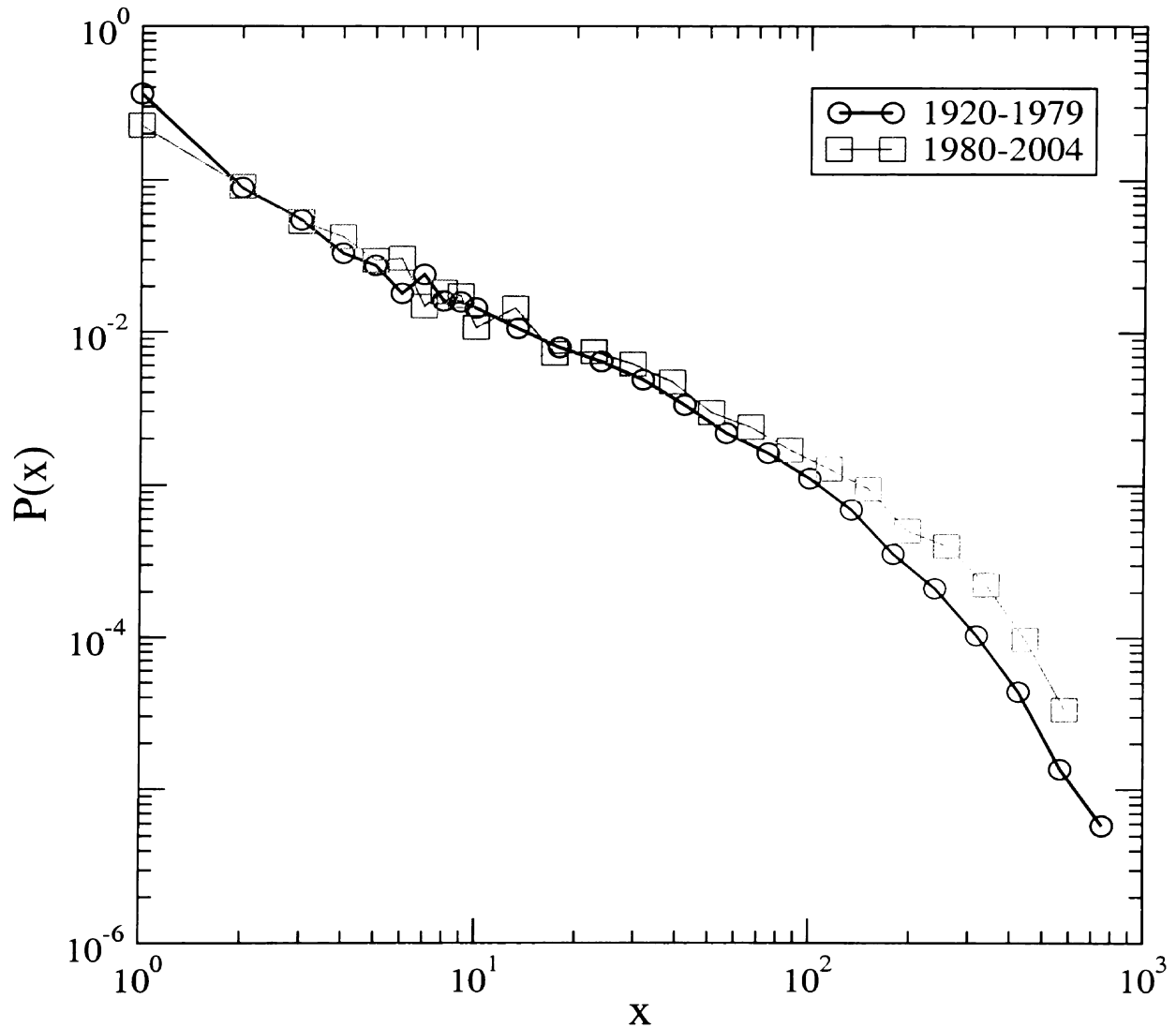
Figure 6.5: Statistical evidence in career home run distributions consistent with performance enhancement drugs. Probability density function of home runs hit over a player's career ending in two different time periods, before and after 1980 (pitchers are excluded). More home runs are being collected in the extreme part of the distribution by individuals ending their careers in the last 25 years, 1980-2004, marked by the "steroids era".
