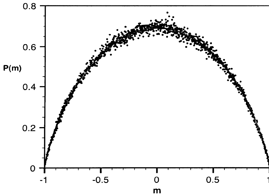
Figure 9.5: Comparison the analytic magnetization distribution for two zealots on the ring (Eq. (9.15)) and simulation results (points).
