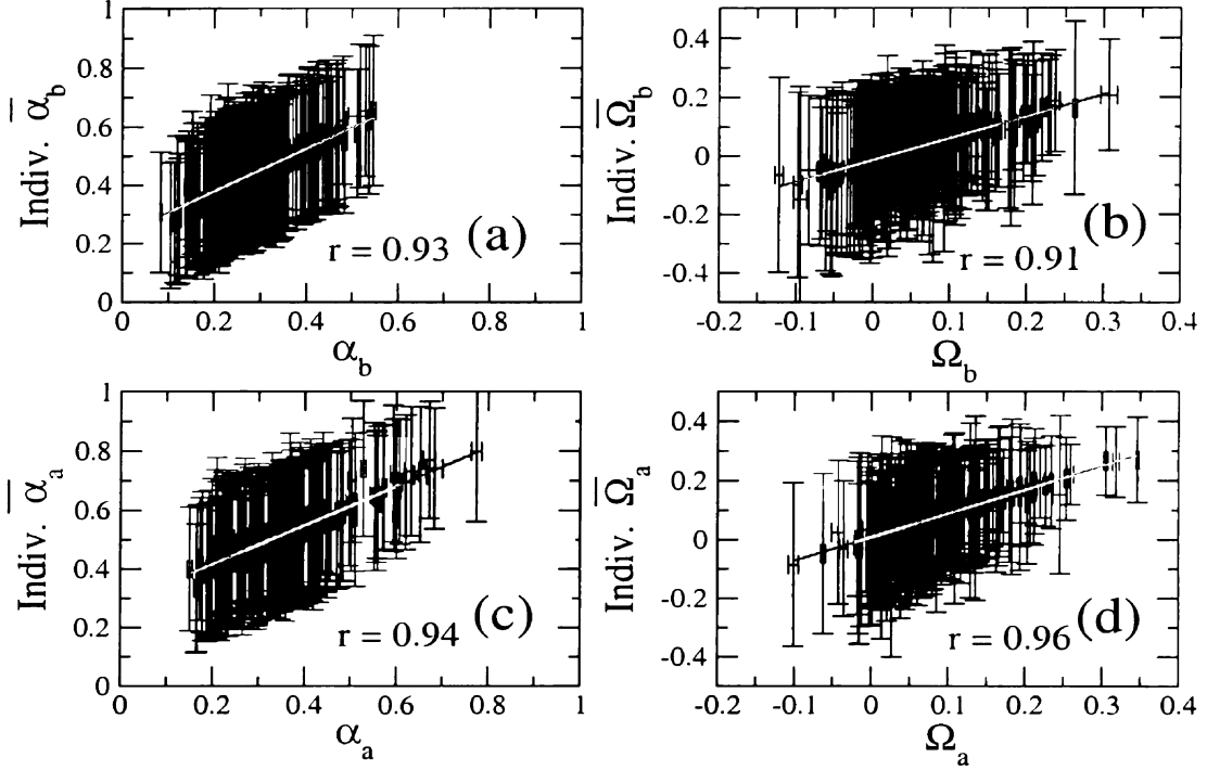
Figure 4.7: In order to account for the dispersion in the pdfs plotted in Figs. 4.6(c) and 4.6(d) for individual stocks, we compare the average values \bar{\alpha}_{a,b} and \bar{\Omega}_{a,b} computed from all N_{a,b}^j(\tau) with the \alpha_{a,b} and \Omega_{a,b} computed from the corresponding average market response N_{a,b}(\tau) for each of the 219 T_c . The visually apparent correlation indicates that the parameters quantifying N_{a,b}(\tau) are a good representation of the average N_{a,b}^j(\tau) . The correlation coefficient r for each linear regression is provided in each panel.
