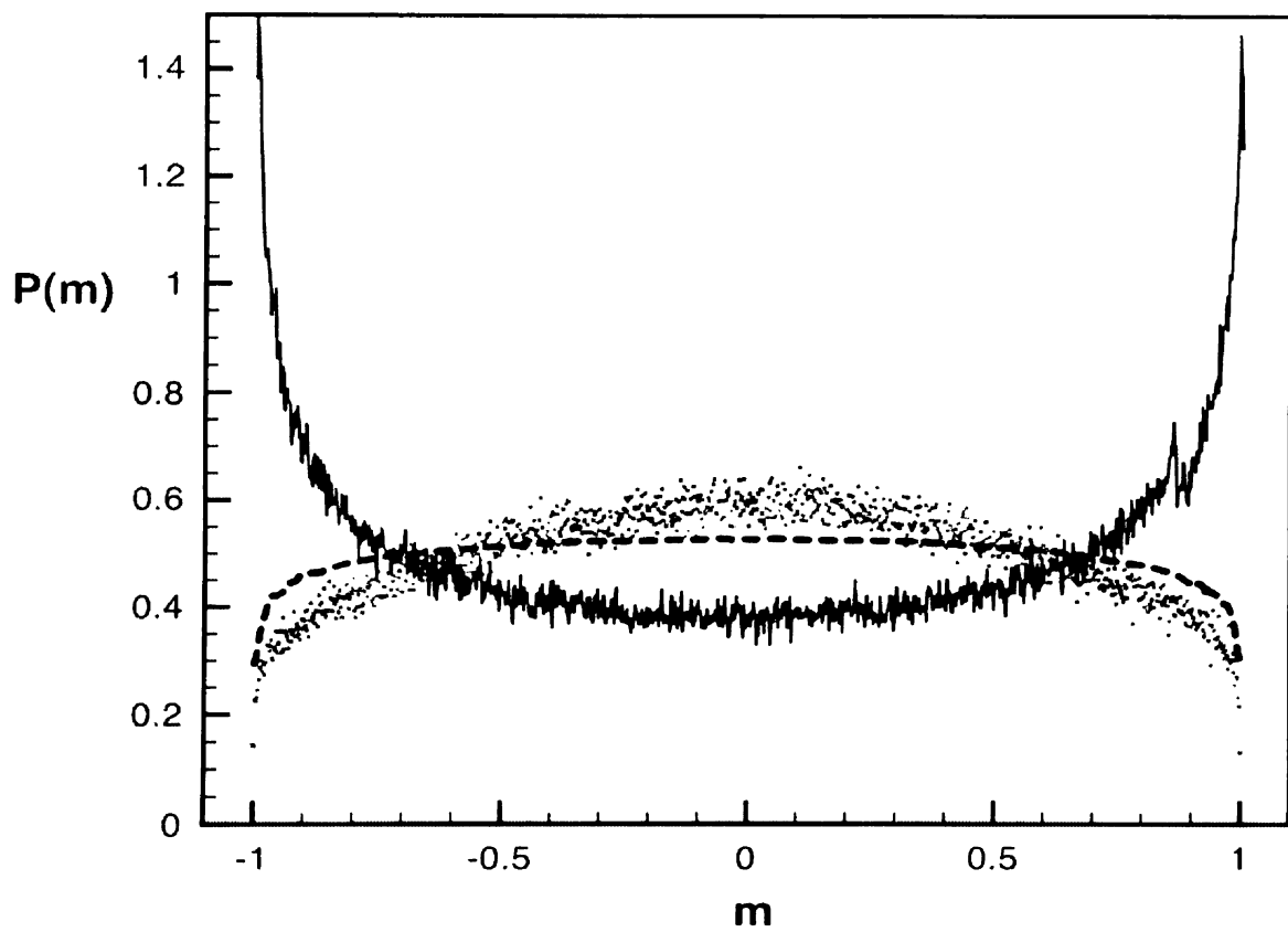
Figure 9.7: Comparison of simulations for the magnetization distribution in two dimensions when the two zealots are adjacent (curve with peaks near \pm 1 ), maximally separated (dots), and averaged over many different zealot configurations (dashed).
