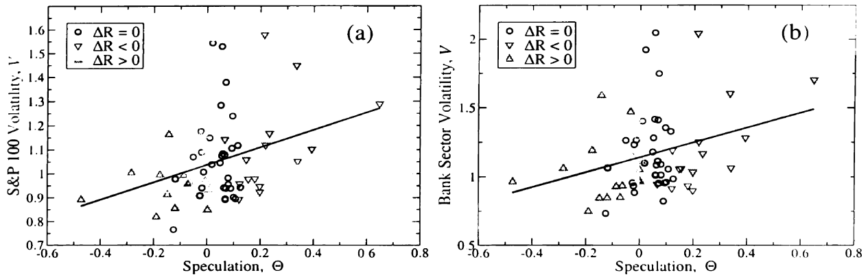
Figure 3.3: Demonstration of the relation between speculation of interest rate change and market volatility in the S&P100 and for the subset of Banking stocks. We relate \Theta_i , the speculation in the market before a FOMC meeting defined in Eq. (3.2), to the market volatility V_i defined in Eq. (3.5). A large absolute value of \Theta_i reflects the high probability that an interest rate change will happen. Interestingly, there are many instances where \Theta_i \approx 0 , followed by large volatility. These values correspond to FOMC decisions to maintain interest rate levels ( \Delta R = 0 ), and suggest a fundamental difference in the dynamics following decisions to change versus decisions not change the Federal Funds Target rate. Also, there is an underlying symmetry in \Delta R , since in the case of either a rate increase or a rate decrease, the FOMC also has the option of no increase. Hence, \Delta R = 0 can occur as either “good” or “bad” news, whereas typically decisions of \Delta R > 0 reflect situations with positive market sentiment whereas decisions of \Delta R < 0 reflect situations with negative market sentiment. Hence, the asymmetry in market volatility is consistent with the “sign effect” [13]. Although the correlation between \Theta_i and V_i is dominated by residual error, it is nevertheless supporting that the regression captures the crossover at (\theta, V) = (0, 1) . Including all data points, the regression correlation coefficient is r^2 = 0.34 , and the slope of the regression is m = 0.36 \pm 0.13 for panel (a) and r^2 = 0.30 and m = 0.54 \pm 0.22 for panel (b). All linear regressions pass the ANOVA F-test, rejecting the null hypothesis that m = 0 at the \alpha = 0.05 significance level.
