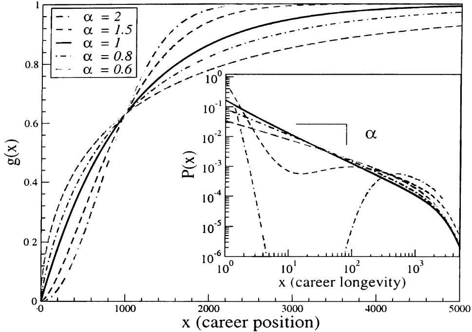
Figure 7.2: A demonstration of the fundamental relationship between the progress rate g(x) and the career longevity pdf P(x) . The progress rate g(x) represents the probability of moving forward in the career to position x+1 from position x . The small value of g(x) for small x captures the difficulty in making progress at the beginning of a career. The progress rate increases with career position x , capturing the role of the Matthew effect. We plot five g(x) curves with fixed x_c = 10^3 and different values of the parameter \alpha . The parameter \alpha emerges from the small- x behavior in g(x) as the power-law exponent in P(x) . ( Inset ) Probability density functions P(x) resulting from inserting g(x) with varying \alpha into Eq. [7.5]. The value \alpha_c \equiv 1 separates two distinct types of longevity distributions. The distributions resulting from concave career development \alpha < 1 exhibit monotonic statistical regularity over the entire range, with an analytic form approximated by the Gamma distribution \text{Gamma}(x; \alpha, x_c) . The distributions resulting from convex career development \alpha > 1 exhibit bimodal behavior. One class of careers is stunted by the difficulty in making progress at the beginning of the career, analogous to a “potential” barrier. The second class of careers forges beyond the barrier and is approximately centered around the crossover x_c on a log-scale.
