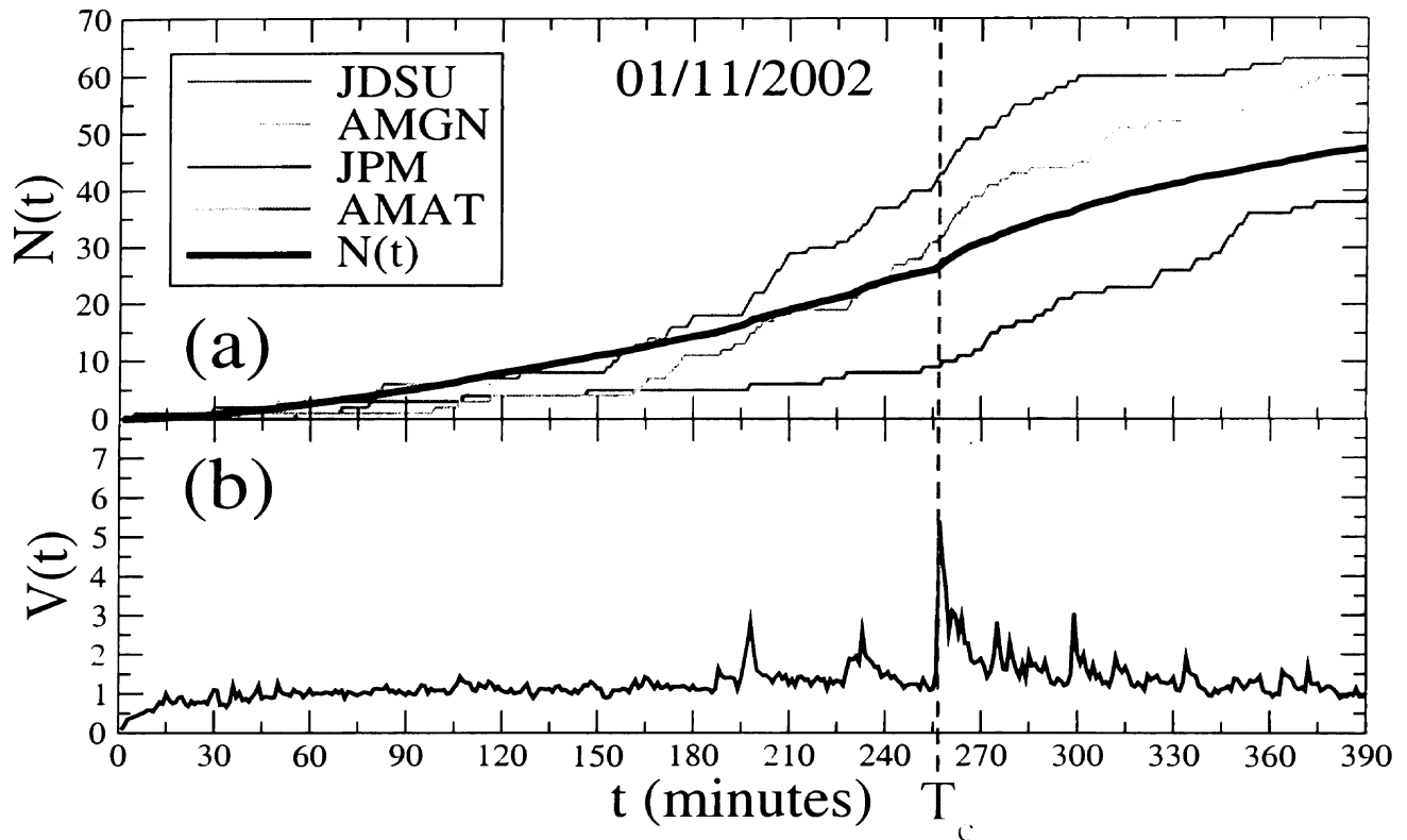
Figure 4.1: Typical volatility curves on 01/11/2002 with market shock at T_c = 256 minutes. (a) The cumulative volatility N^j(t) for the stock of several large companies have varying behavior before T_c , but each stock shown begins to cascade soon after T_c . The market average N(t) over all S = 531 stocks analyzed demonstrates a distinct change in curvature at t = T_c . (b) The average market volatility V(t) demonstrates a sharp peak at T_c , and also two precursor events at t \approx 190 and t \approx 230 minutes.
