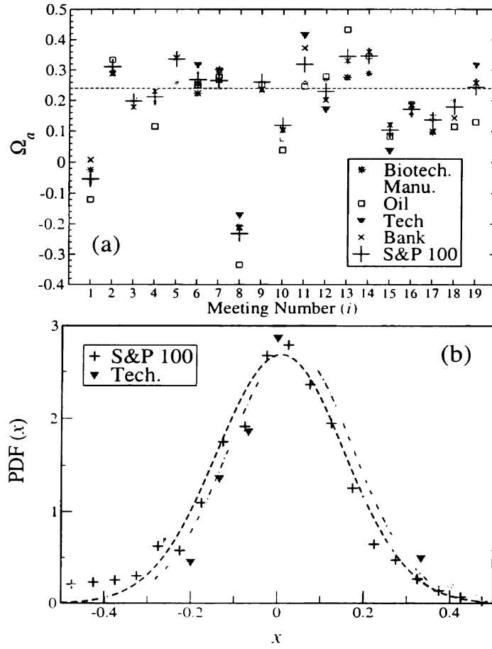
Figure 3.8: (a) A comparison of \Omega_a for 5 sectors with volatility threshold q = 3 suggests a broad universal market response to FOMC news. The Tech sector tends to have the largest average \Omega_a , where large \Omega values corresponds to faster relaxation. The horizontal straight line represents the mean \bar{\Omega}_a = 0.24 \pm 0.08 , averaged over all stocks in the S&P100 and all scheduled meetings (excluding the unscheduled meetings i = \{1, 4, 8\} ). (b) Probability density function P(x) of the variable x \equiv x_{a,i}^j = \Omega_{a,i}^j - \langle \Omega_{a,i} \rangle , which correspond to individual \Omega_{a,i}^j values centered around the average exponent \langle \Omega_{a,i} \rangle of a given meeting i . Tech sector Omori exponents are larger on average, and since larger \Omega values correspond to shorter relaxation time, we find that the Tech sector stocks responds more quickly to FOMC news, possibly as a result of relatively intense trading activity among these stocks.
