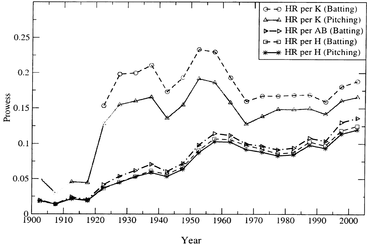
Figure 6.4: Average league prowess \langle P \rangle calculated for 5-year periods starting in 1900. The trendline for HR/AB has been multiplied by a factor of 4 for clarity. The difference in the trendlines for Hr per Hit for batter and pitcher are essentially constant over the years. Following from the form of our weighted average, this suggests that the changes in home run prowess are not due to fluctuations in the talent pool arising from expansion dilution. If more home runs were being hit by veteran batters against poor pitching, then a spread would appear, assuming that poor pitchers don't stay at the major league level very long. Instead, we see that veteran hitters (with a large fraction of the total hits) are hitting more home runs off of veteran pitchers (with a large fraction of hits surrendered, and thus many innings pitched).
