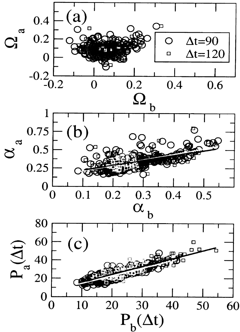
Figure 4.11: A comparison of Omori parameters before and after T_c for N(\tau) and varying \Delta t indicate that \alpha_b and P_b(\Delta t) are better conditional estimators for the dynamics after T_c . (a) Weak relationship between \Omega_b and \Omega_a for \Delta t = 90 and 120. (b) Strong relationship between \alpha_b and \alpha_a for \Delta t = 90 and 120, with both linear regressions passing the ANOVA F-test at the p < 0.001 confidence level. (c) Strong relationship between P_b(\Delta t) and P_a(\Delta t) for \Delta t = 90 and 120 min. at the p < 0.001 confidence level.
