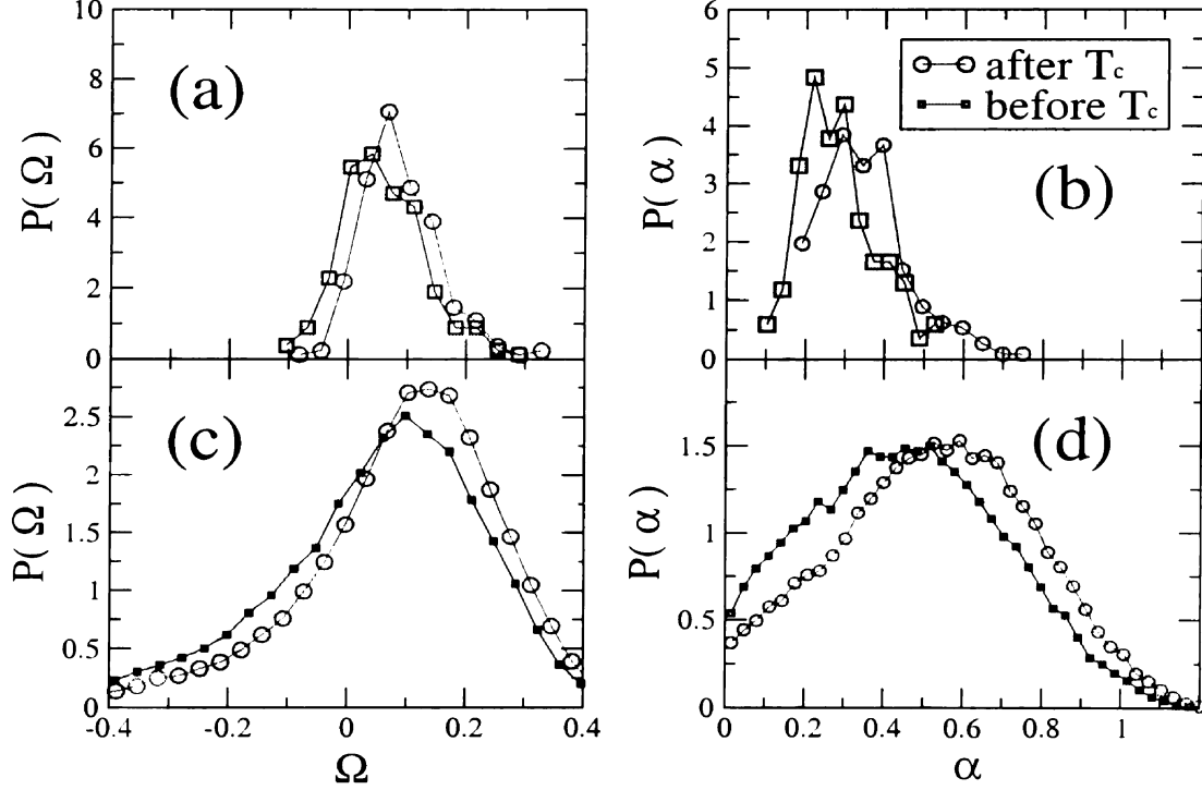
Figure 4.6: (a,b) Comparison of the probability density functions P(\alpha) and P(\Omega) of Omori parameters \alpha and \Omega computed from the average market response N_{a,b}(\tau) . (c,d) The analogous pdf plots computed from individual stock response N_{a,b}^j(\tau) . The average and standard deviation of each data set are (a) \Omega_a = 0.09 \pm 0.07 , \Omega_b = 0.06 \pm 0.07 (b) \alpha_a = 0.35 \pm 0.11 , \alpha_b = 0.28 \pm 0.09 (c) \Omega_a = 0.08 \pm 0.20 , \Omega_b = 0.03 \pm 0.22 and (d) \alpha_a = 0.53 \pm 0.25 , \alpha_b = 0.46 \pm 0.24 . Values of both \Omega_a and \alpha_a are consistently larger than \Omega_b and \alpha_b , indicating that the response time after T_c is shorter than the activation time leading into T_c . However the response cascade after T_c has, generally, a larger amplitude.
