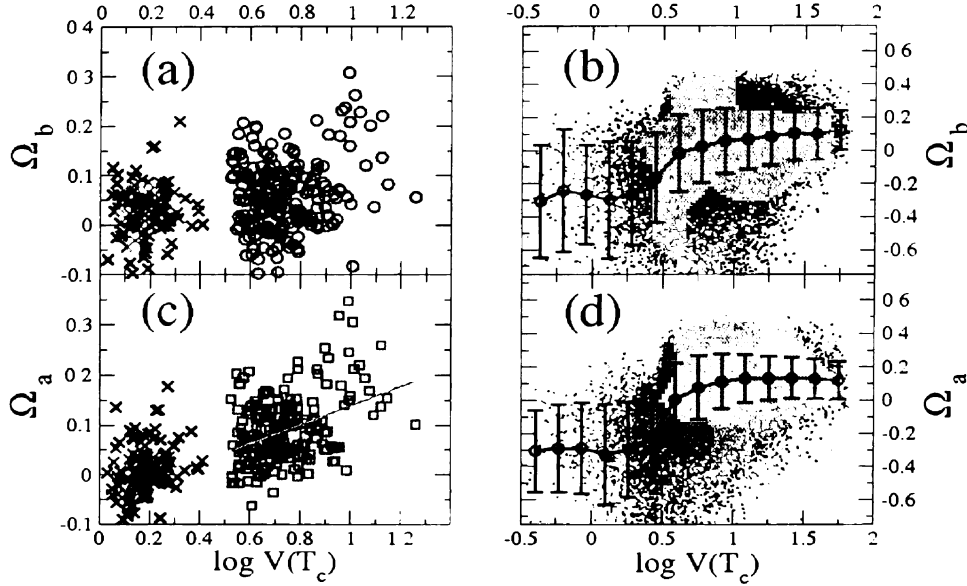
Figure 4.8: The relation between the magnitude M \equiv \log V(T_c) and the Omori exponents \Omega_{a,b} . In panels (a) and (c) we compare values calculated from the average market response N_{a,b}(\tau) , and in panels (b) and (d) we compare values calculated from individual stock response N_{a,b}^j(\tau) . (a) Weak relation before T_c , where we validate the linear regression model at p = 0.001 significance level, but with correlation coefficient r = 0.22 . The dispersion may result from the variability in anticipation preceding the market shock at T_c . (c) The relation between \Omega_a and M is stronger after T_c than before T_c , with linear regression significance p \approx 0 , correlation r = 0.40 , and regression slope m = 0.19 \pm 0.03 . The increasing trend demonstrates that a faster response, quantified by larger \Omega_a , follows a larger M . Data points in panels (a) and (c) denoted by the symbol \times correspond to values of \Omega_{a,b} calculated for randomly selected T_c on those 118 days analyzed without a single value of x(t) > x_c . In panels (b) and (d) there is much dispersion in the \Omega values of individual stocks for given V(T_c) . However, the average trends demonstrate a significant crossover at M_x \approx 0.5 from \Omega_{a,b} < 0 to \Omega_{a,b} > 0 . The case of \Omega < 0 can occur when there is more volatility clustering for large \tau than for small \tau , whereas the case of \Omega > 0 occurs for large volatility cascading around \tau \gtrsim 0 . This crossover could result from the difference between anticipated and surprise shocks at T_c .
