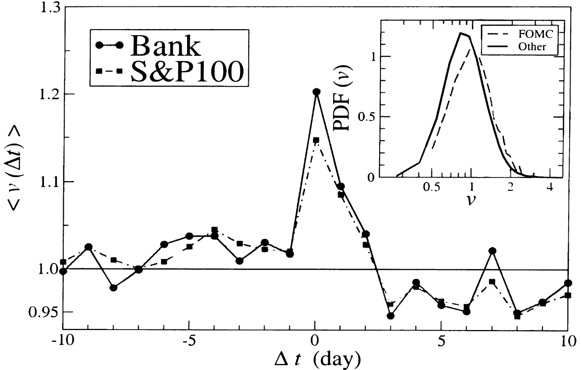
Figure 3.2: Average daily volatility trend defined in Eq. (3.4) exhibits increased market volatility on the day of FOMC meetings, corresponding to \Delta t = 0 . “Bank” refers to the portfolio of 18 stocks that belong to the S&P100. There is a 15-20% increase in volatility on days corresponding to FOMC meetings. Standard deviation \sigma(v(\Delta t)) \approx 0.4 can be assigned to each data point in the time series, and are calculated by randomizing the daily volatility time series of each company. (Inset) Probability density function (pdf) of normalized volatility v \equiv r(t)/\langle r \rangle , where the quantity r(t) \equiv \ln(p_{hi}(t)/p_{low}(t)) is the range of the price time series of a given stock for a particular day. We plot the pdf of volatility values for the S&P100 on the set of days with FOMC meetings and for the set of all “other” days. The distributions are approximately log-normal, with a shift towards higher average volatility on FOMC days. The average values for the two data sets are \langle v \rangle_{FOMC} = 1.12 and \langle v \rangle_{other} = 1.00 .
