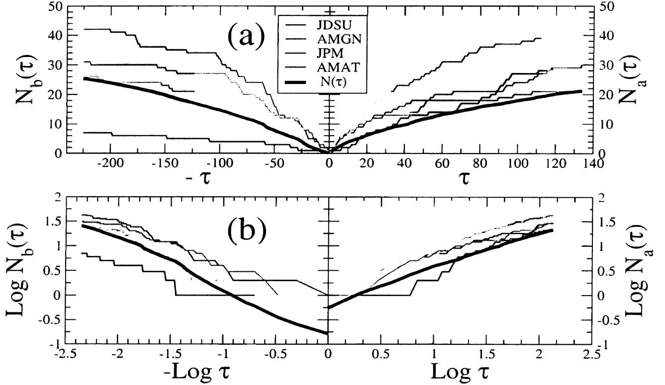
Figure 4.2: (a) An illustration of N_b(\tau) and N_a(\tau) for the same set of curves plotted in Fig. 4.1. The displaced time \tau = |t - T_c| is defined symmetrically around T_c = 256 minutes on 01/11/2002. (b) \log N_b(\tau) and \log N_a(\tau) are linear with \log \tau over two orders of magnitude on a logarithmic scale. The Omori parameters in Eq. (4.5) calculated from N(t) are \Omega_b = 0.09 \pm 0.01 , \alpha_b = 0.21 \pm 0.01 and \Omega_a = 0.32 \pm 0.01 , \alpha_a = 0.81 \pm 0.01 .
