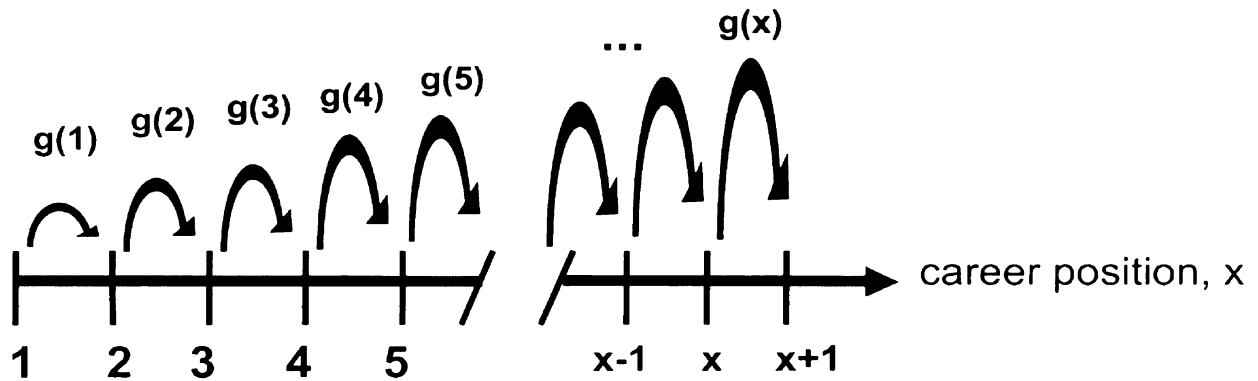
Figure 7.1: Graphical illustration of the stochastic Poisson process quantifying career progress with position-dependent progress rate g(x) . A new opportunity, corresponding to career position x + 1 , can refer to a day at work or, even more generally, to any assignment given by an employing body. In this framework, career progress is made at a rate g(x) that is slower than the passing of work-time, representing the possibility of career stagnancy. The traditional Poisson process corresponds to a constant progress rate g(x) \equiv \lambda . Here, we use a functional form for g(x) \equiv 1 - \exp[-(x/x_c)^\alpha] that is increasing with career position x , which captures the salient feature of the Matthew effect, that it becomes easier to make progress the further along the career.
