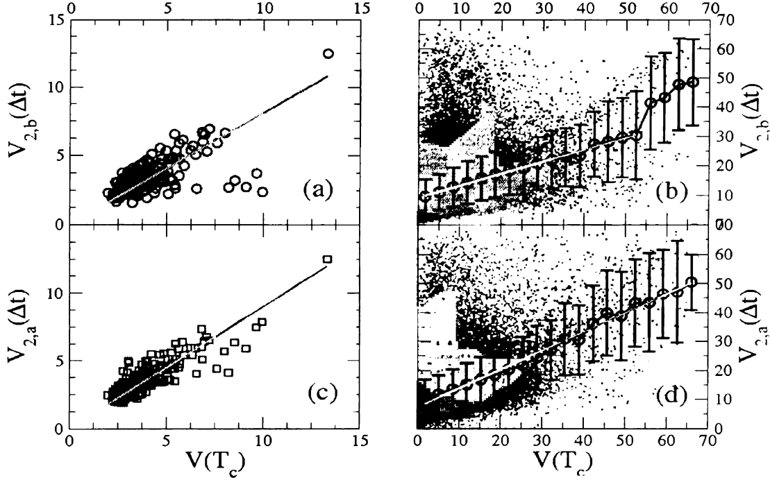
Figure 4.12: The increasing relation between the size of the main shock V(T_c) and the size of the second largest aftershock (or preshock) V_2(\Delta t) within \Delta t minutes of T_c demonstrates that the volatility of the largest aftershock (or preshock) increases with mainshock volatility. As with the Bath law for earthquakes, we observe a proportional relation V_{2,a}(\Delta t) \equiv C_B V(T_c) which corresponds to a Bath parameter B = -\log C_B . For the average market response N_{b,a}(\Delta t) we calculate C_B for (a) the dynamics before, C_B = 0.81 with correlation coefficient r = 0.70 and \chi^2 = 212 , and for (c) the dynamics after C_B = 0.9 with r = 0.87 and \chi^2 = 109 . For the Bath law corresponding to individual stocks we find that a linear function best fits the relation between V(T_c) and the average value \bar{V}_2(\Delta t) calculated for equal-sized bins as indicated by circles with one standard deviation error bars. We calculate the regression slope for the Bath law (b) before is m = 0.65 \pm 0.02 and (d) after is m = 0.40 \pm 0.01
