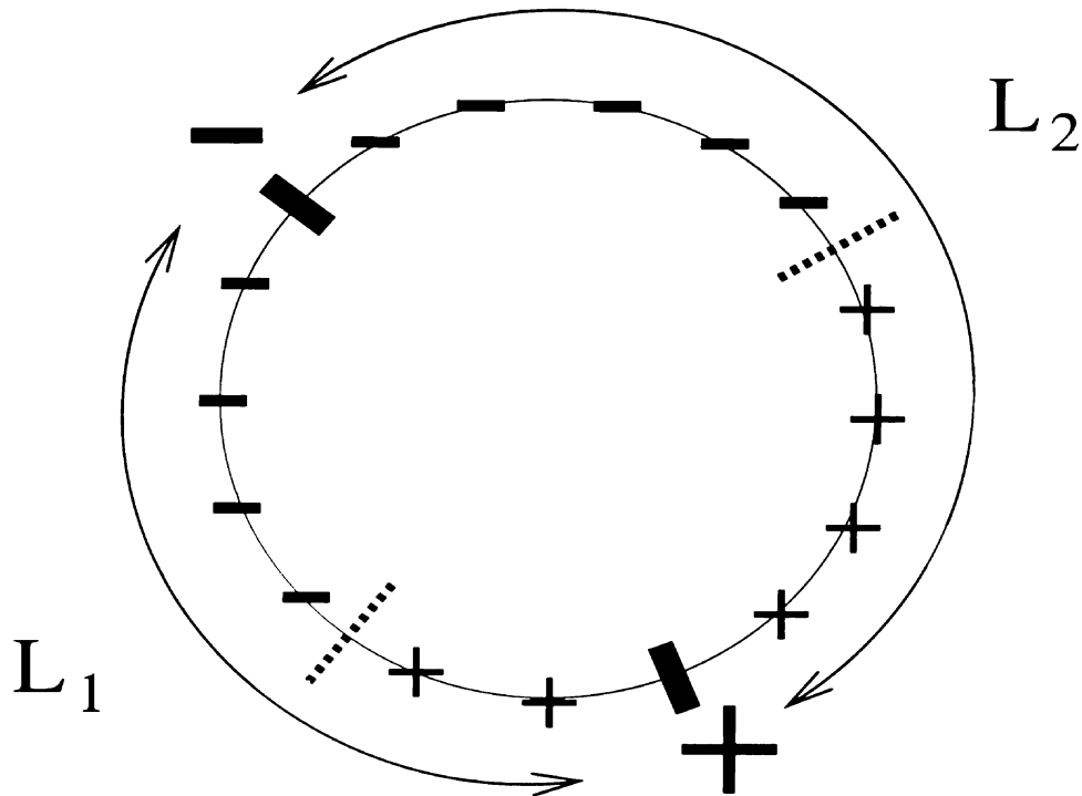
Figure 9.3: A ring divided into two independent segments by oppositely-oriented zealots (thick lines). Also shown is the state of each voter and the domain wall in each segment at long times (dotted lines).
