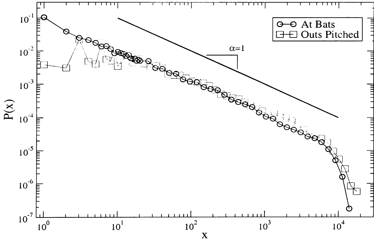
Figure 6.1: Probability density function of player longevity. Longevity is defined as the number of outs-pitched (pitchers), and the number of at-bats (all batters) for players ending their career in the years 1920-2000. Power law extends over more than three orders of magnitude, with \alpha \approx 1 . For reference: straight line represents the power-law P(x) \sim x^{-1} .
