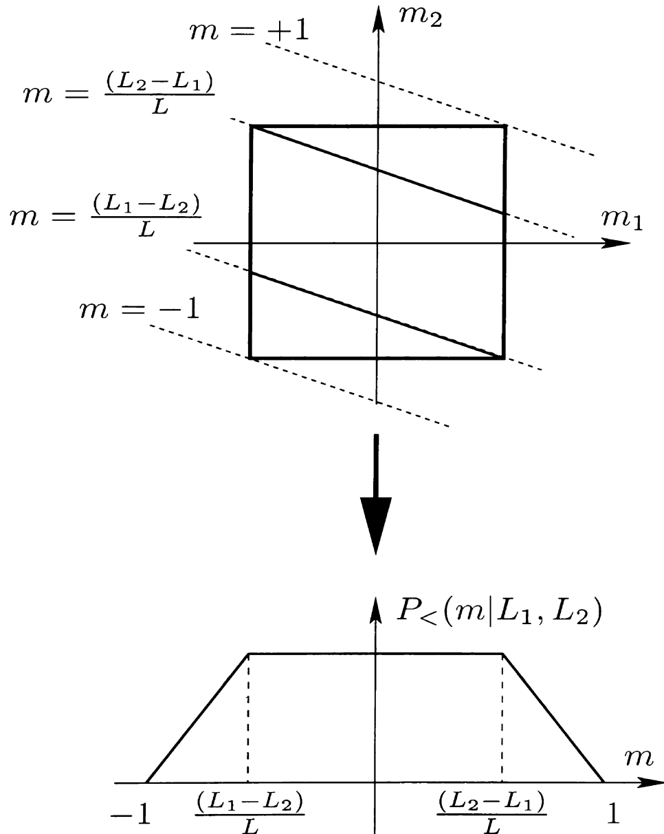
Figure 9.4: (Top) Rays of fixed magnetization (dashed) for the case L_1 < L_2 . The probability for a given value of m is proportional to the length of the ray corresponding to this m value within the unit square (solid). (Bottom) The resulting magnetization distribution P_<(m|L_1, L_2) for a given L_1 and L_1 < L_2 .
