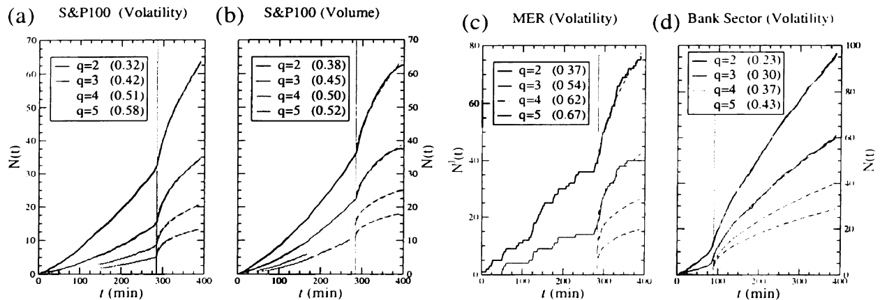
Figure 3.4: The cumulative volatility time series N(t) demonstrates Omori-law response dynamics, here in response to FOMC announcements occurring at the time T indicated by a vertical solid line. The abrupt change in the curvature of N(t) around time t \approx T illustrates the increased volatility caused by the announcement. The significant aftershocks which occur until the end of the trading day are consistent with “market underreaction” [12, 13]. Market underreaction and other market inefficiencies can result from increased levels of uncertainty among traders following market news [14]. Each time series N(t) is calculated for a given volatility threshold q , where larger q values correspond to N(t) curves with smaller amplitude (smaller rate of large volatility events). Panels (a,b,c) illustrate the dynamics around a scheduled announcement made at T = 285 minutes (2:15 PM ET). For the S&P 100, we calculate N(t) on 05/15/01 for (a) 1-minute volatility and (b) 1-minute total volume using Eq. (3.8). (c) We calculate N^j(t) for Merrill Lynch (MER) on 08/21/01. (d) The Omori law also occurs for unscheduled FOMC announcements, as illustrated for the Bank sector N(t) on 04/18/01, when the surprise rate change was announced at T = 90 minutes (11:00 AM ET), resulting in raised levels of volatility throughout the entire trading day. For panels (a-d), the dashed lines are power-law fits beginning immediately after the announcement, with the corresponding exponents \Omega_n(q) appearing in parentheses within the legends.
